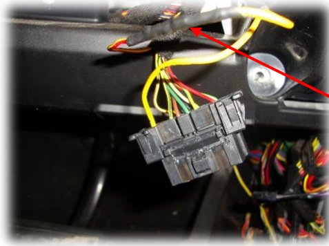
Vehicle harness wire (red/yellow, left) connected to remaining loose wire of disarm module harness (yellow, right) and heat shrink applied
